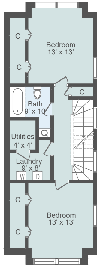
Second Floor
