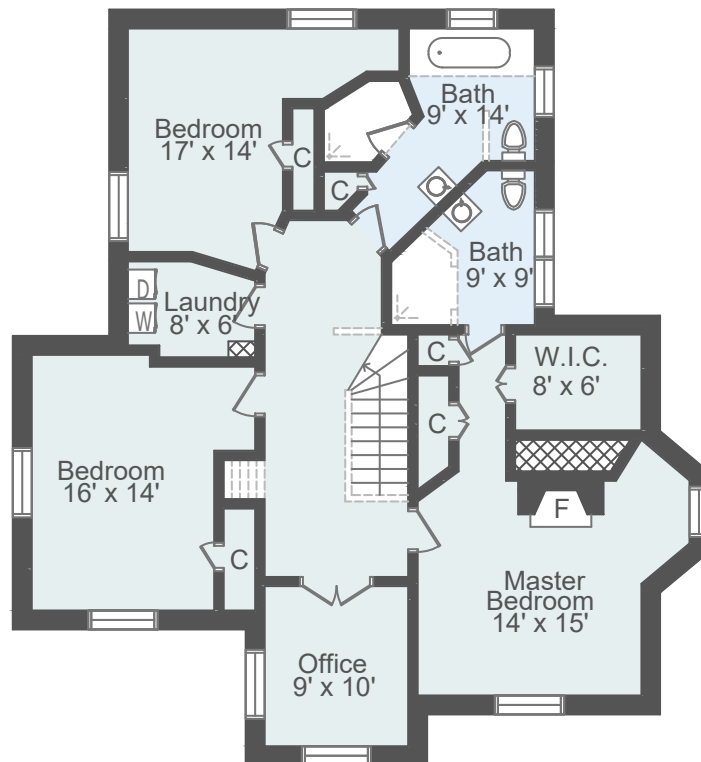
Third Floor
